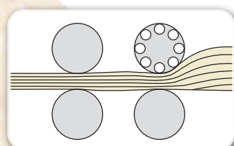
B 麵皮打薄整麵 Dough Sheet Pressing & Sheeting
