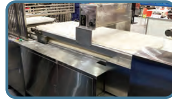
麵帶對折 Dough Sheet Folding in half
