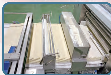
麵帶層次&麵帶延壓 Laminating & Sheeting
